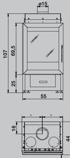
PORTA PIANA FLAT DOOR PORTE PLATE PUERTA PLANA
