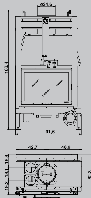
BIFACCIALE DOUBLE-FRONTED DOUBLE FAÇADE BIFACIAL
